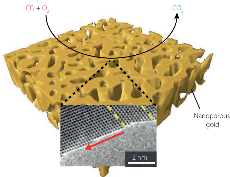
Gold atoms migrate at right angles (red arrow) to a planar ‘twin’ interface (yellow lines) during the oxidation of carbon monoxide on nanoporous gold.
