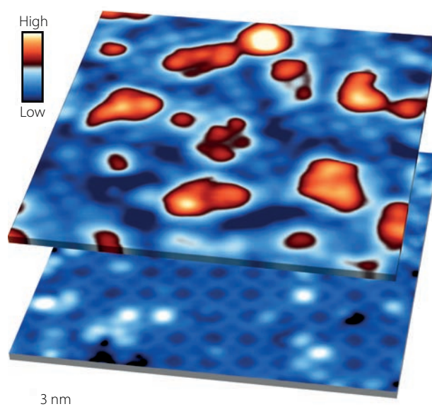
Scanning tunneling microscopy images of strontium oxide ( \text{SrO}_x ) islands (red, top) after deposition of \text{SrO} on a titanium–oxygen surface (bottom).
