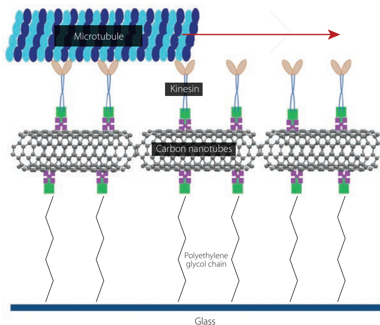
Multiwalled carbon nanotubes attached to a glass plate act as a track for a kinesin-powered microtubule conveyor belt.
