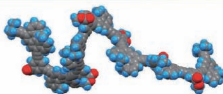
Helical oligomers
